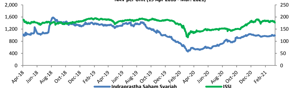
NAV per Unit (19 Apr 2018 - Mar. 2021)
